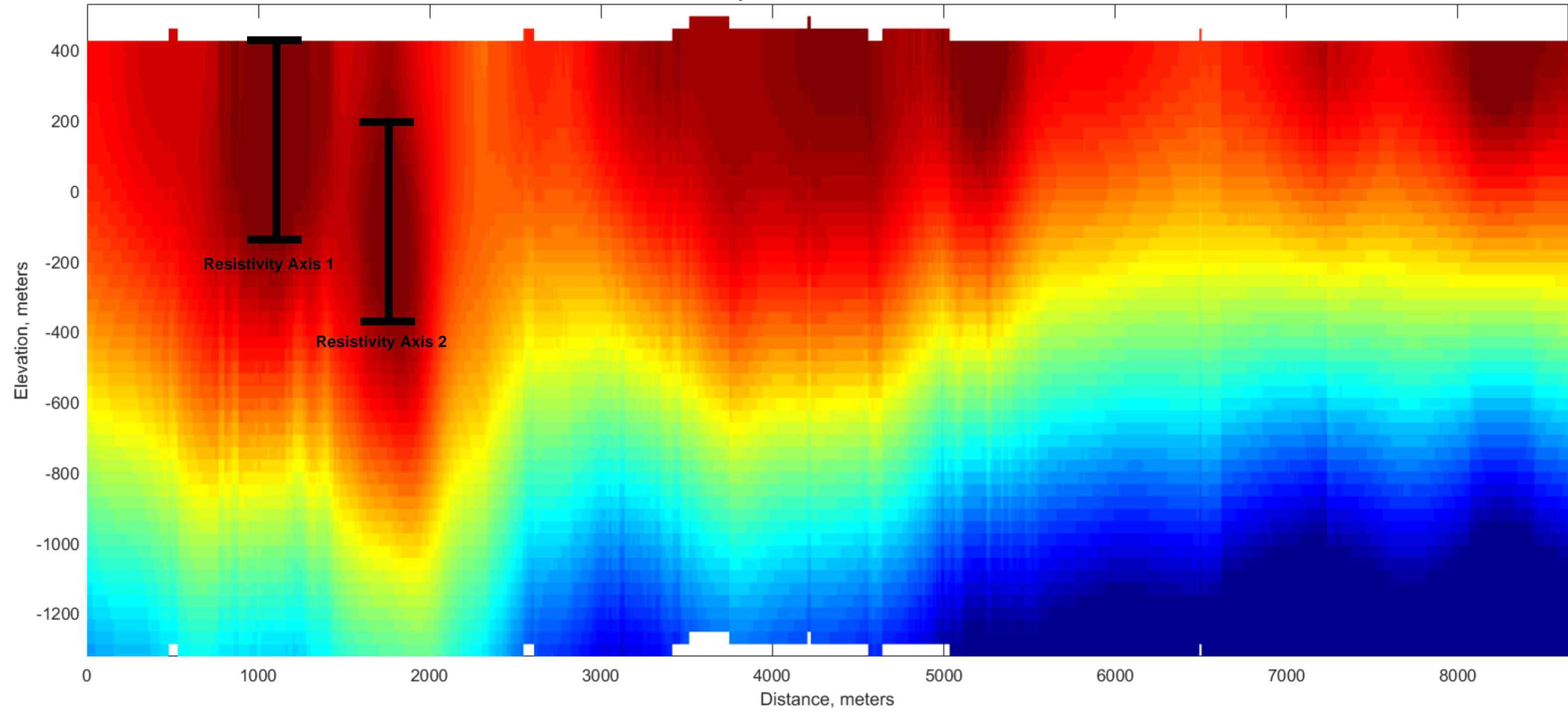
Resistivity of inverted section Line--3840
