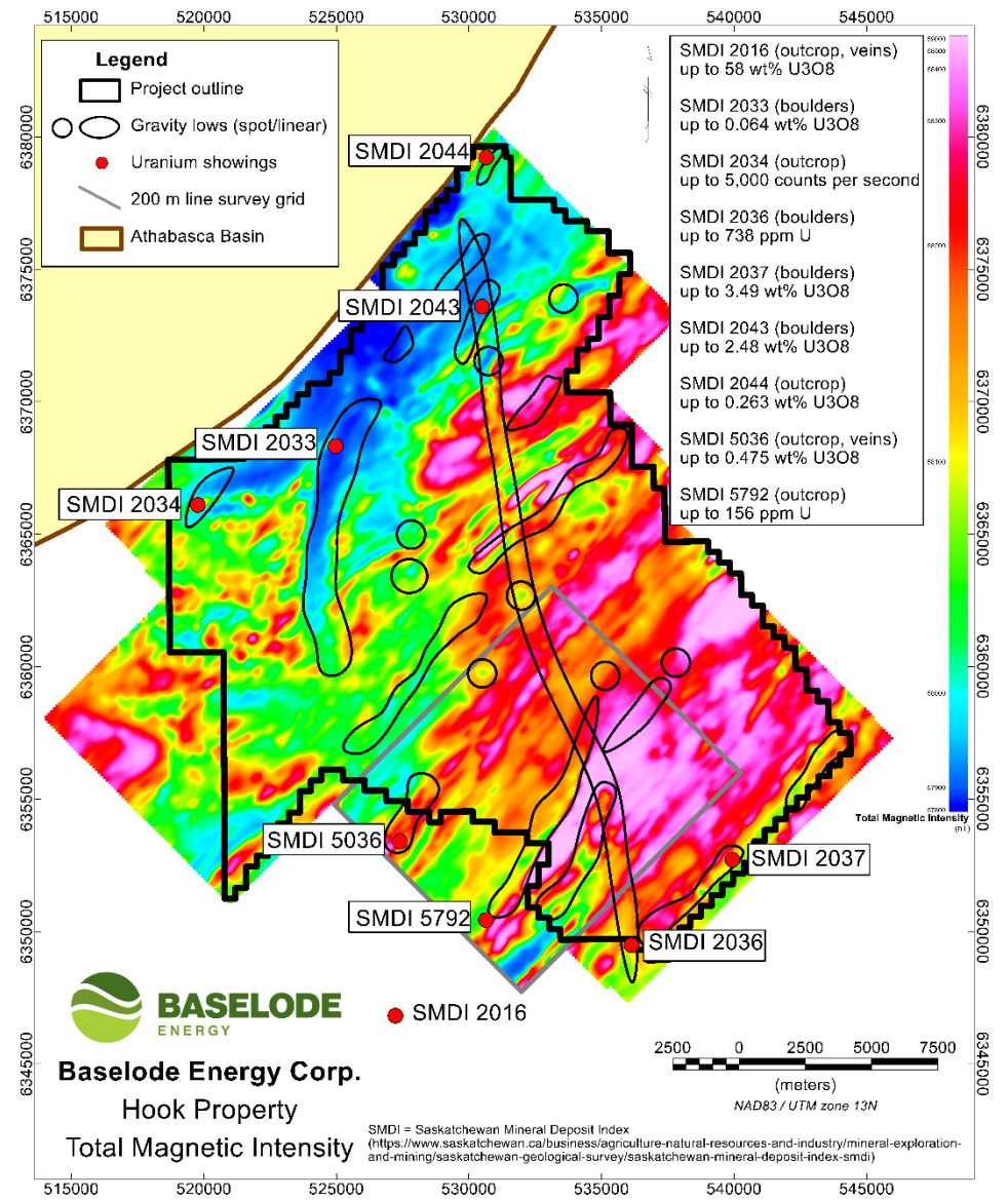
Figure 2: Gravity low targets over airborne magnetics background
