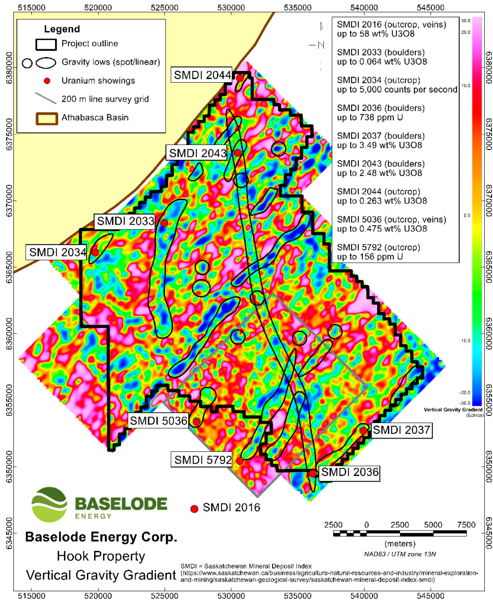
Figure 1: Gravity low targets over airborne gravity background
